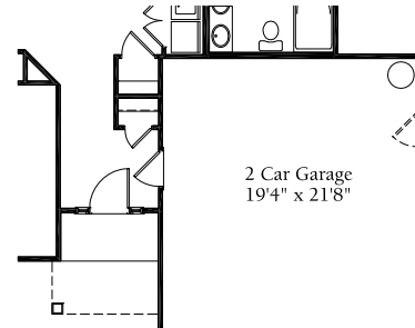
First Floor Plan with Optional 2 Car Garage
