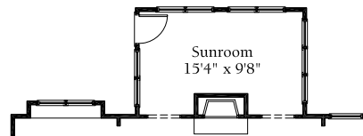
Optional Sunroom with Fireplace in Great Room
